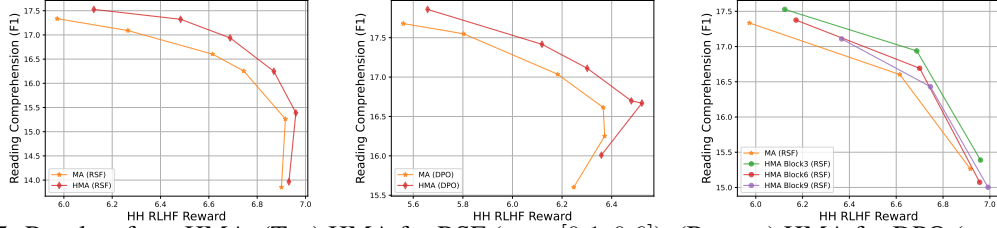
Figure 5: Results of our HMA. (Top) HMA for RSF ( \alpha \in [0.1, 0.6] ), (Bottom) HMA for DPO ( \alpha \in [0.1, 0.6] ). (Right) HMA for RSF with different choices of K . Refer to Appendix E.5 for more results.
