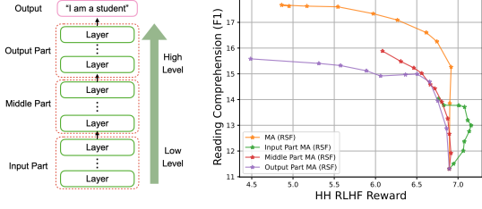
Figure 4: (Left) Illustration of proof of concept experiments. We divide the Transformer into 3 parts. We only average one part each time. (Right) Merging different parts of the transformers.
