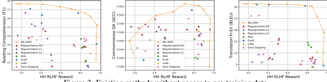
Figure 3: Existing methods without access to pre-training data
