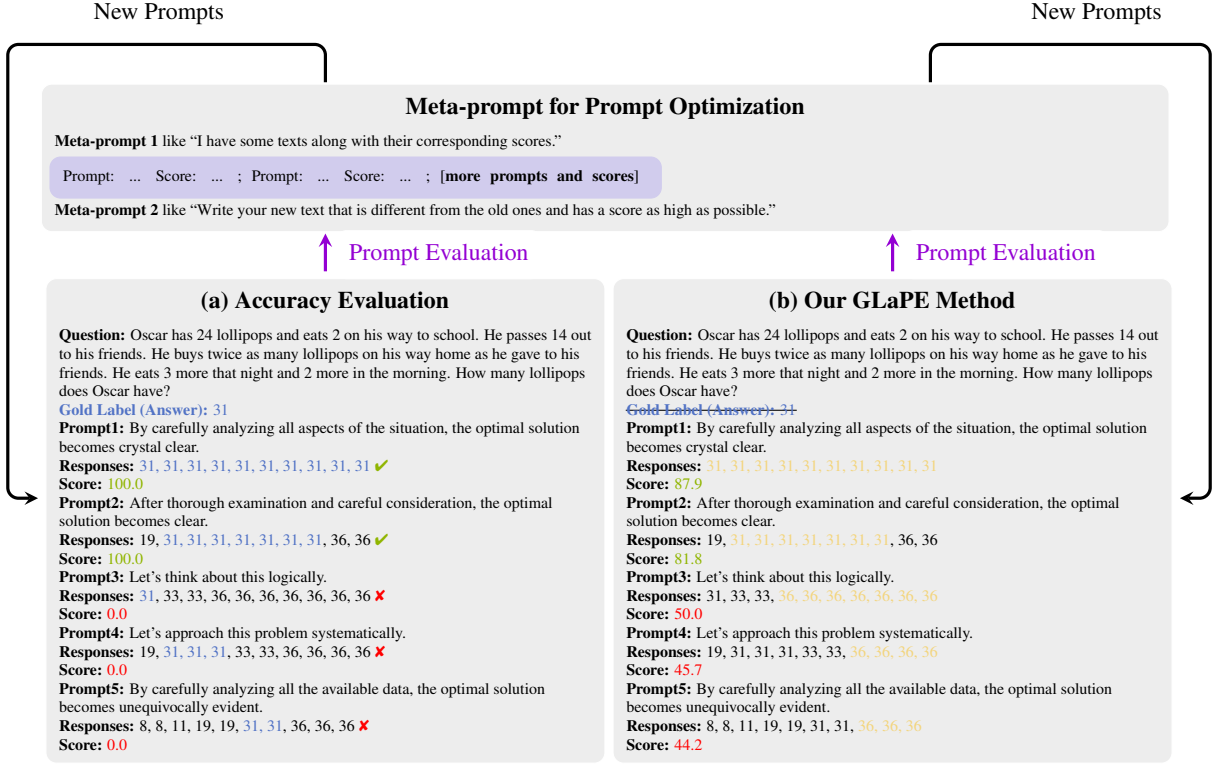
Figure 1: Sketch of prompt optimization utilizing the LLM as an optimizer (Yang et al., 2023), featuring distinct prompt evaluation metrics based on: (a) accuracy or (b) our proposed GLaPE. The texts are favorably read in colors. Blue : gold label, Yellow : most frequent answer, Green : high score, Red : low score, Purple : prompt evaluation.
