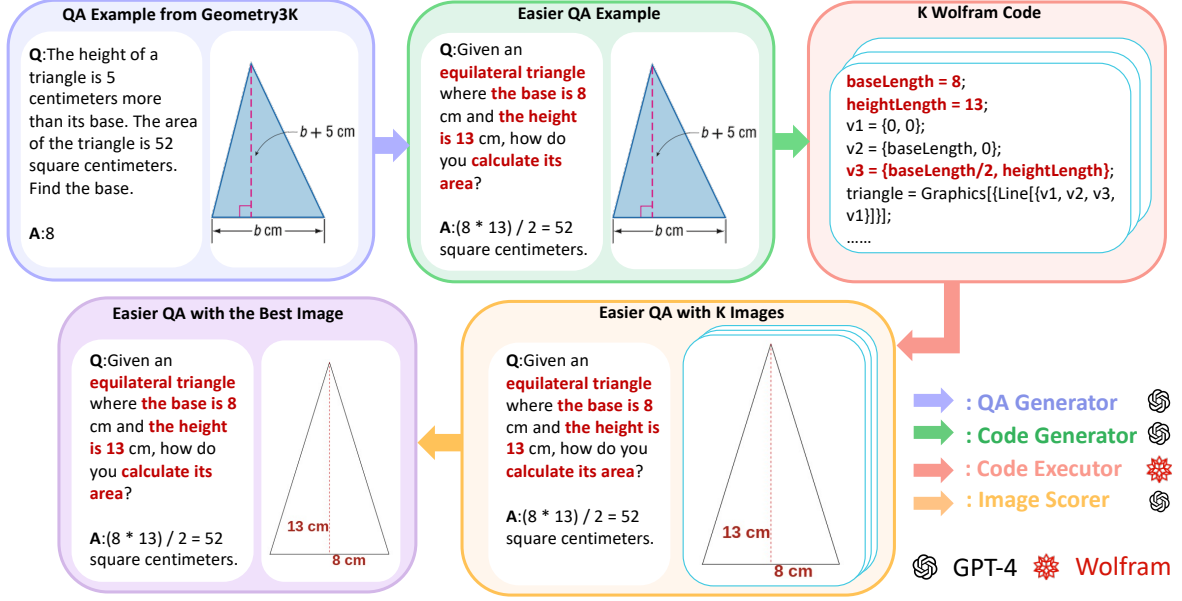
Figure 1: Pipeline of our geometric data generation. During the first step, we employ GPT-4V to generate simplified geometric question-answer pairs based on open-source datasets. We highlight the simplified parts compared to the original questions. During the second step, we employ GPT-4 to generate K Wolfram code for each question-answer pair. During the third step, we execute K code to obtain K images. During the fourth step, we employ GPT-4V to score the degree of alignment between the generated images and the questions. We choose the image with the highest score. Finally, we can obtain simplified and image-text matching geometric problems.
