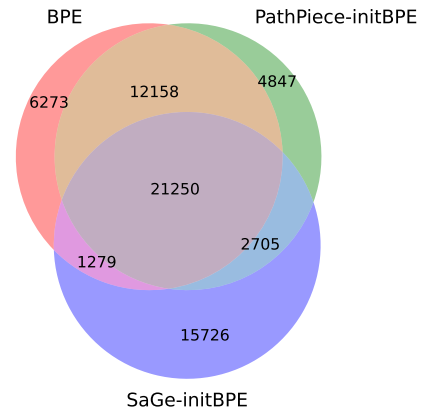
Figure 5: Venn diagram comparing 40,960 token vocabularies of BPE, PathPieceL and SaGe – the latter two were both initialized from a BPE vocabulary of 262,144.
