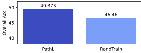
Figure 17: Comparison of PathPieceL and RandTrain, with BPE initial vocab, and FirstSpace pre-tokenization, p=0.0137
