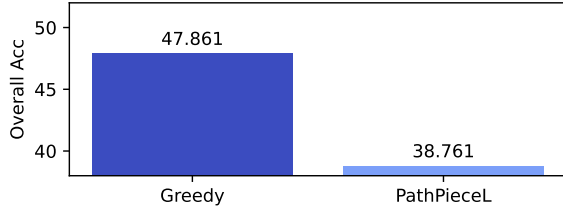
Figure 16: Comparison of Greedy and PathPieceL segmentation, with RandTrain vocabulary construction, n -gram initial vocab, and FirstSpaceDigit pre-tokenization, p=0.00293
