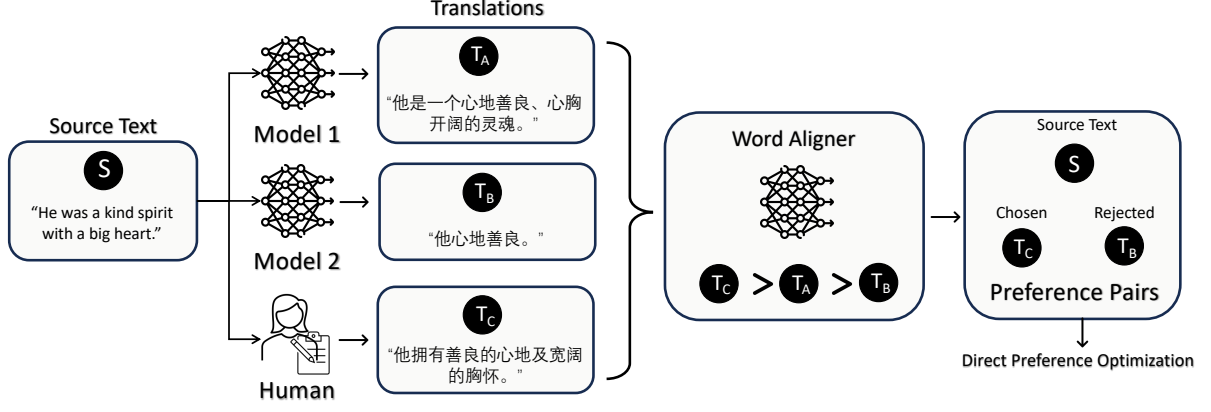
Figure 2: An illustration of WAP framework. The source is first translated by multiple MT tools, including human translation. An external word aligner is then utilized to predict the coverage score for each translation. Finally, translation with the highest and lowest coverage score are selected as preference pairs for preference optimization.
