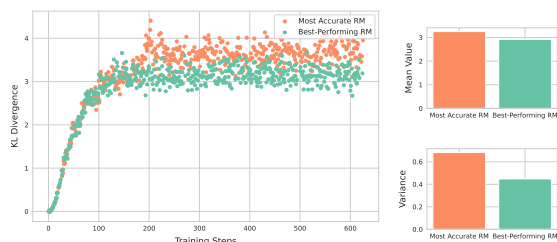
Figure 7: Relevance task KL divergence (T5-small model): training steps vs. KL divergence (left), mean and variance of rewards (right).
