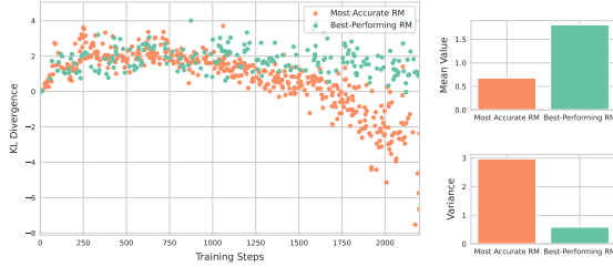
Figure 23: Factuality task KL divergence (T5-base model): training steps vs. KL divergence (left), mean and variance (right).
