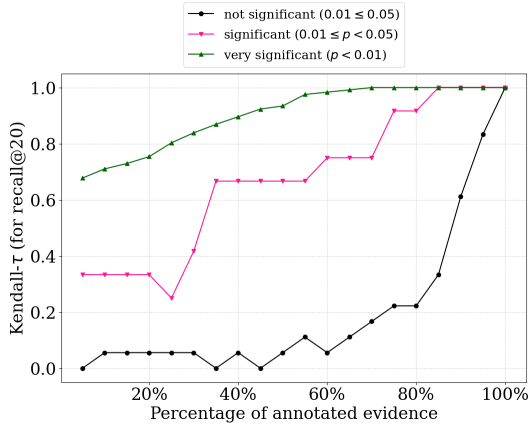
Figure 3: Partial-Kendall- \tau between rankings of systems with k percent annotations and ranking with all evidence, using recall@20 . System pairs are divided into 3 buckets as described in Section 3.3.
