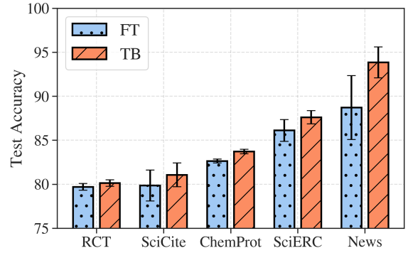
Figure 5: Domain Specific Language Modeling. TempBalance demonstrates significant performance gain when training the RoBERTa-base model on five low-resource domain-specific datasets.
