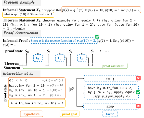
Figure 1: Problem Example : An input example from Zheng et al. (2022). Proof Construction : A sequence of tactics updates the state interactively to prove the goal. Interaction at S_0 : Given the value of \sigma^{-1} , the goal is to prove the value of \sigma . rw fails to rewrite the proof goal with h_1 . simp fails to simplify the proof goal with existing hypotheses. The have tactic successfully proves h_3 reversely by observing the goal. It corresponds to the color sentence in the informal proof.
