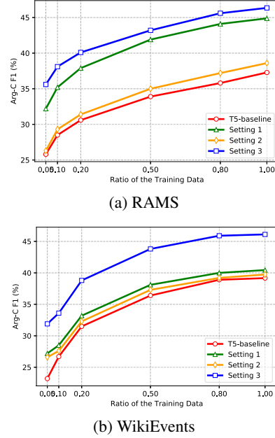
Figure 6: Arg-C F1 scores with different training data ratios on both benchmarks.
