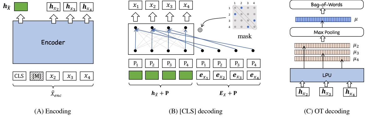
Figure 2: Framework of DupMAE. The unified encoder generates the contextualized embeddings for the [CLS] and ordinary tokens (OT). The [CLS] decoding reconstructs the original sentence leveraging an one-layer transformer; the OT decoding predicts the BoW feature of the input on top of the linear projection unit (LPU) and max-pooling.
