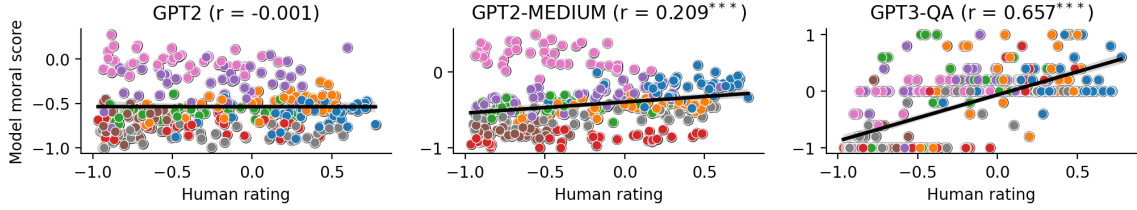
Figure 7: Degree of alignment between the moral scores from EPLMs and fine-grained empirical moral ratings for different topics across countries taken from the World Values Survey (top) and PEW survey (bottom). Each dot represents a topic-country pair. The x-axis shows the fine-grained moral ratings from the ground truth and the y-axis shows the corresponding inferred moral scores. Similar topics in the World Value Surveys are shown with the same color.
