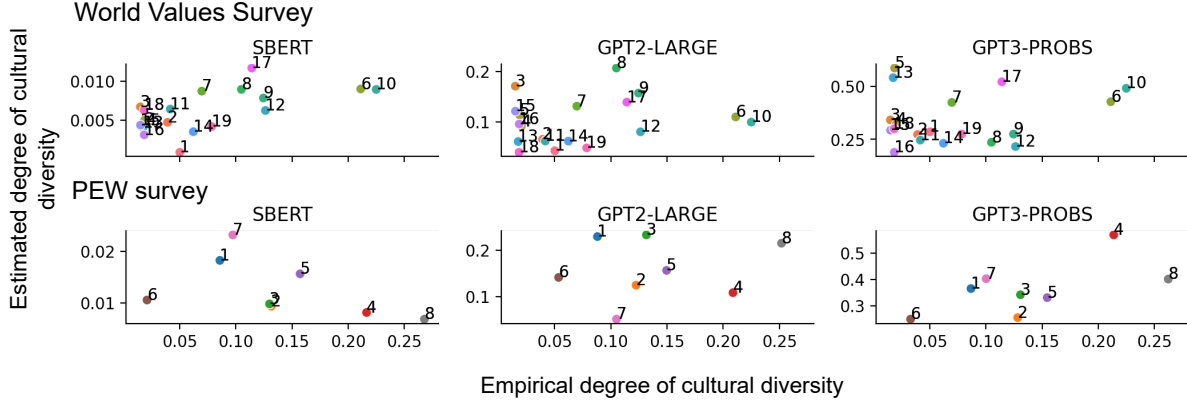
Figure 5: Comparison between the degrees of cultural diversities and shared tendencies in the empirical moral ratings and language-model inferred moral scores. Each dot corresponds to a moral topic. The numerical indices are consistent with the legend indices in Table 5. The x-axis shows the empirical standard deviations in moral ratings across countries and the y-axis shows the standard deviations from the model-inferred moral scores.
