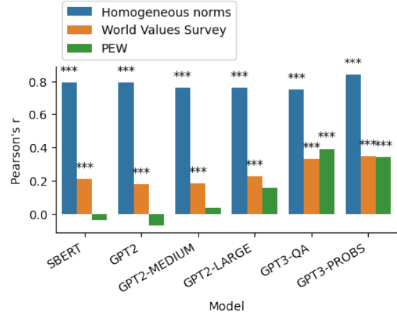
Figure 2: Performance of EPLMs (without cultural prompts) on inferring 1) English moral norms, and 2) culturally diverse moral norms recorded in World Values Survey and PEW survey data. The asterisks indicate the significance levels (“*”, “**”, “***” for p < 0.05, 0.01, 0.001 respectively).
