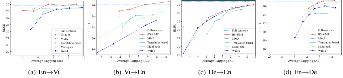
Figure 4: Translation performance of different methods on \text{En} \leftrightarrow \text{Vi} and \text{De} \leftrightarrow \text{En} tasks. It shows the results of our BS-SiMT method, Wait- k policy, Multi-path, Translation-based policy, MMA policy, and the Full-sentence translation model.
