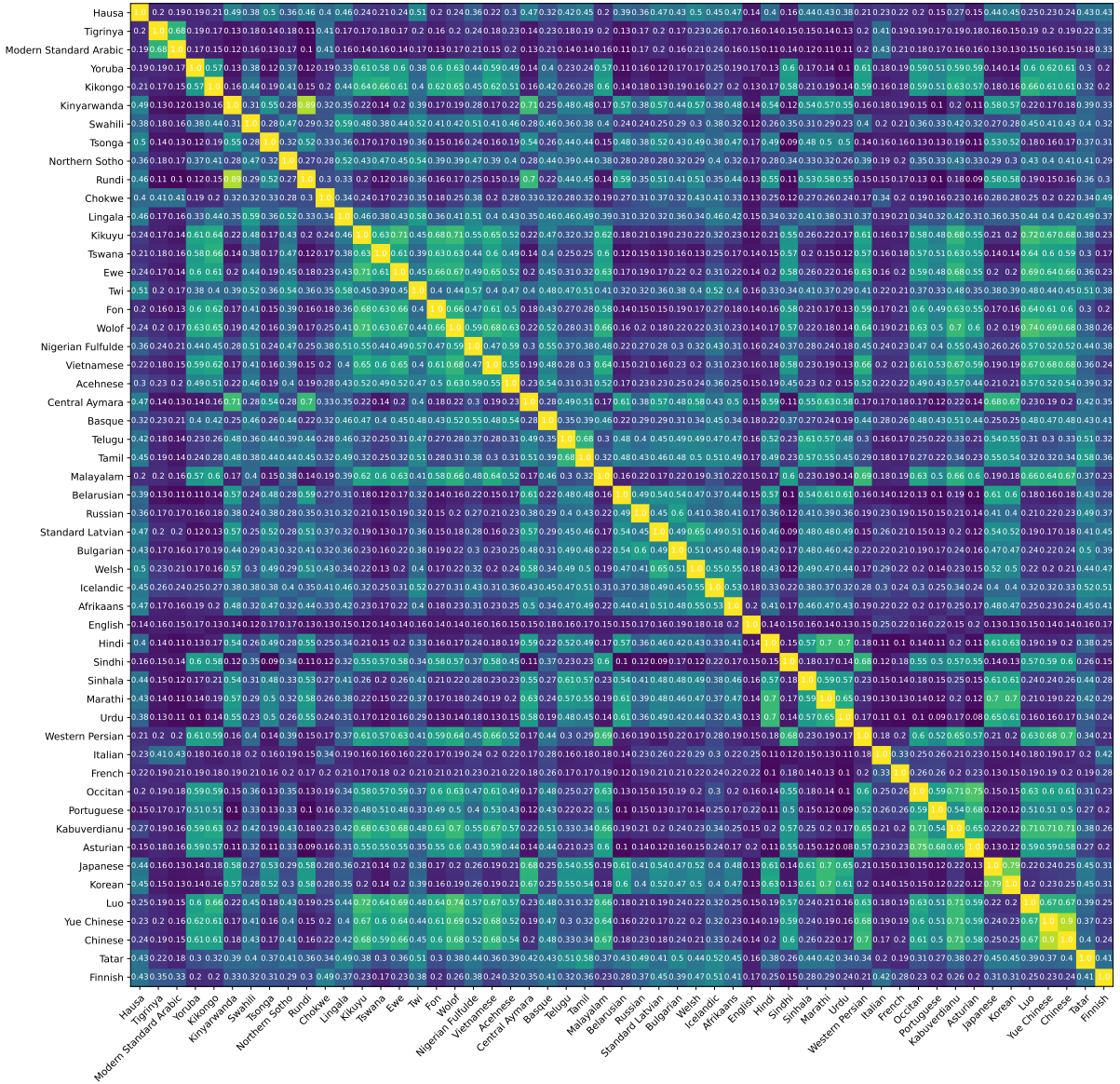
Figure 5: Jaccard similarity of selected 25% decoder experts for different languages. Pruning was done per language with the importance metric and enc/dec threshold pruning. Languages are sorted by language family.
