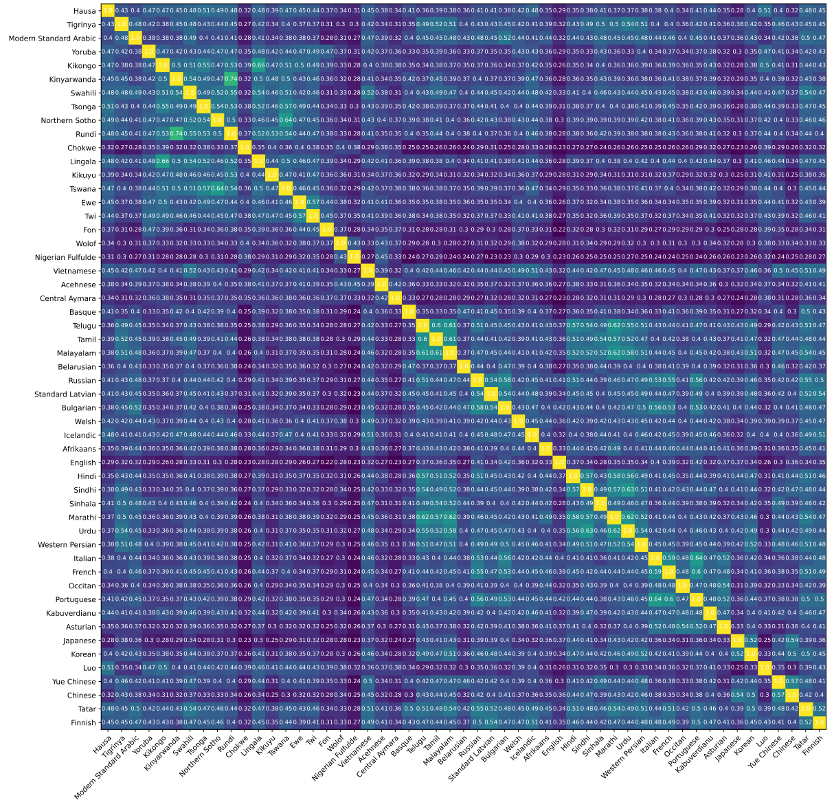
Figure 6: Jaccard similarity of selected 25% encoder experts for different languages. Pruning was done per language with the importance metric and enc/Dec threshold pruning. Languages are sorted by language family.
