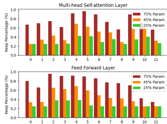
Figure 5: The kept weight for IWSLT’14 De→En.
