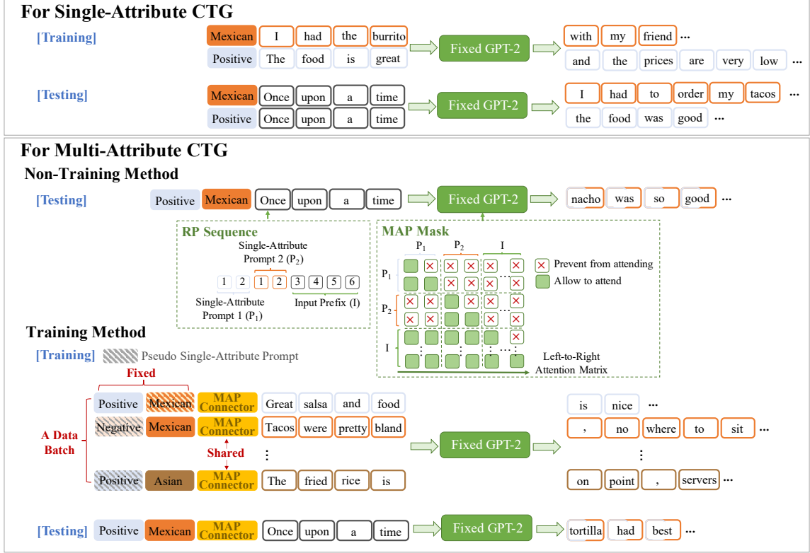
Figure 2: The overview of Tailor to attribute-based CTG. We use 2-token-sized single-attribute prompts for illustration. Notably, the different colored text boxes denote different attribute-specific sentences. For multi-attribute sentences, we use bi-colored text boxes to highlight them.
