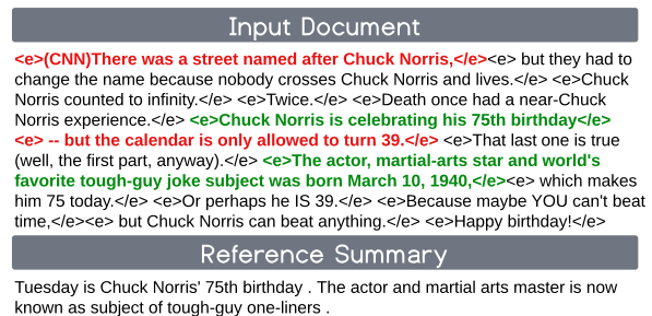
Figure 1: EDU Plan-Guided Abstraction (PGA). EDU spans form the oracle content plan, while EDU spans form a random distractor plan. A model is trained to generate the reference only when given the oracle plan, not the random one. EDU-level plans afford more fine-grained control than sentence-level as irrelevant content is cut out: “but the calendar is only allowed to turn 39”.
