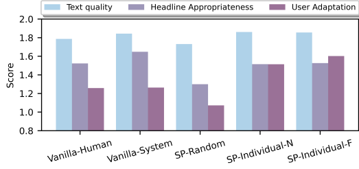
Figure 3: Result of human evaluation scores on the generated headlines w.r.t. text quality, headline appropriateness, and user adaptation.
