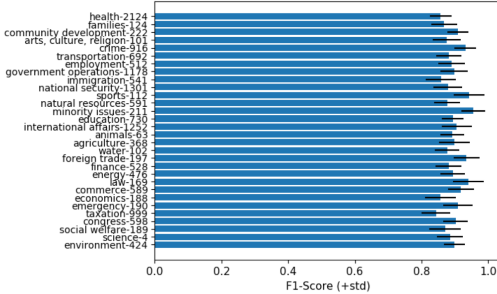
Figure 10: Error Analysis: We report the F1-Score for each bill topic. Bill topics are selected according to the official denomination of the U.S. Congress. We report each topic using the convention TopicName-TopicCode
