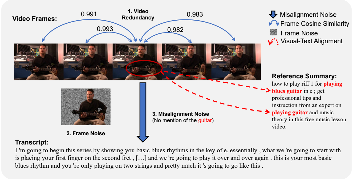
Figure 1: An example of redundancy and noise in a video. As illustrated, consecutive frames have high cosine similarity, which results in a problem of redundancy . In addition, useless information like distracting background and weak alignment between frames and transcripts compose noises in videos.
