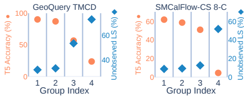
Figure 4: Properties of test example groups, where grouping is based on NoFT prediction outcome: (1) Top-K succeeds; (2) Cover-LS succeeds; (3) only Cover-LS succeeds; and (4) both fail.
