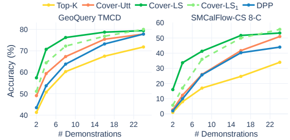
Figure 3: Comparing model accuracy (NoFT setup) based on the number of demonstrations, with multiple methods for selecting demonstrations.
