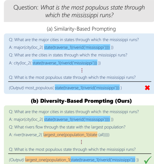
Figure 1: Compositional generalization setup: (a) Selecting demonstrations by considering only similarity to the input yields repetitive demonstrations that do not cover the structures in the target program. (b) However, choosing diverse demonstrations enables better coverage and leads to a correct prediction.
