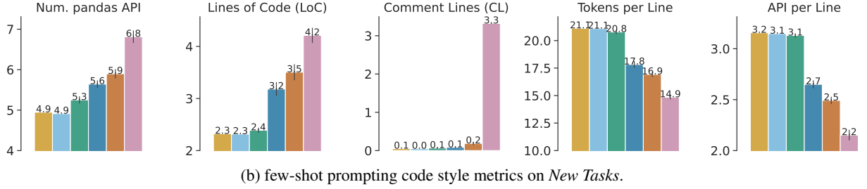
Figure 11: Plots for few-shot prompting evaluation on New Tasks .
