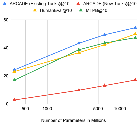
Figure 5: Scaling curve of CODEGEN mono models on ARCADE and existing code generation benchmarks. Results on HumanEval are selected from the best temperature t \in \{0.2, 0.6, 0.8\} (Nijkamp et al., 2022).
