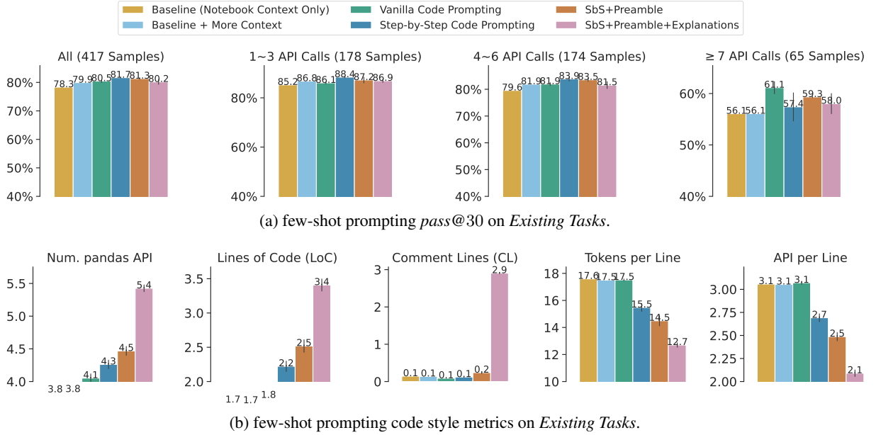
Figure 12: Plots for few-shot prompting evaluation on Existing Tasks .
