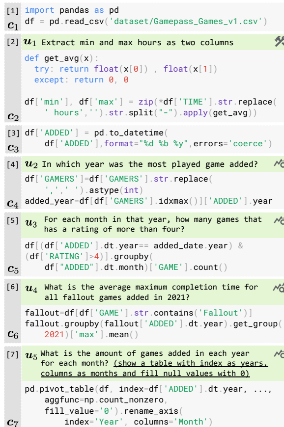
Figure 1: An example of a computational notebook adapted from our dataset, with examples of reading data (cell c_1 ), data wrangling ( c_2, c_3 ), and exploratory data analysis ( c_4 \sim c_7 ). Annotated NL intents ( u_i ) are shown in green.
