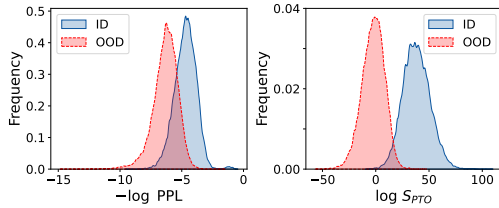
Figure 2: Histogram of the OOD detection score from PPL (left) and PTO (right) on IMDB-Yelp.
