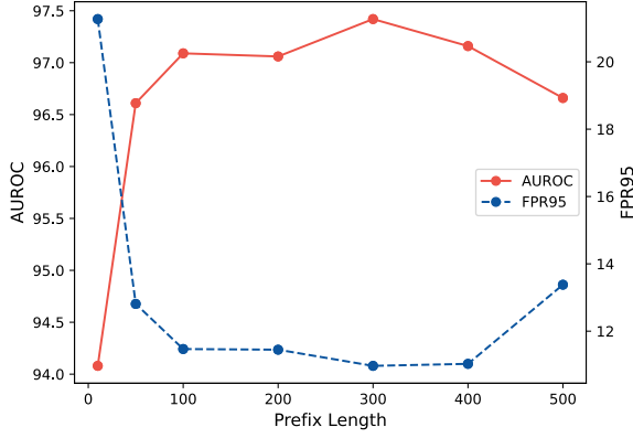
Figure 4: AUROC and FPR95 of PTO under different prefix lengths on the IMDB-Yelp validation set.
