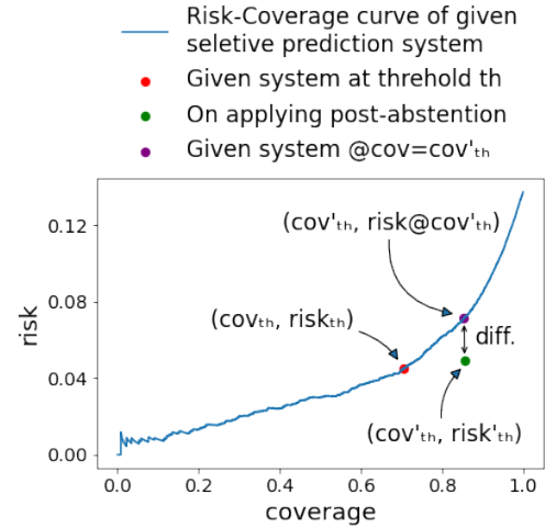
Figure 2: Summarizing performance evaluation methodology of post-abstention. Given a selective prediction system with coverage cov_{th} and risk risk_{th} at abstention threshold th , let the new coverage and risk after applying a post-abstention method be cov'_{th} and risk'_{th} respectively. From the risk-coverage curve of the given system, we calculate its risk at coverage cov'_{th} and compare it with risk'_{th} (diff). For the method to have a positive impact, risk'_{th} should be lower than the risk of the given system at coverage cov'_{th} .
