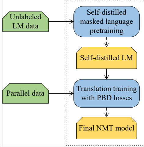
Figure 1: Overall training flow of pretrained bidirectional distillation for machine translation.
