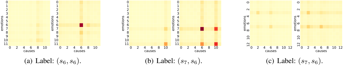
Figure 7: Accurate match of JCB (right graphs) for emotions and causes compared with PBJE (left graphs).
