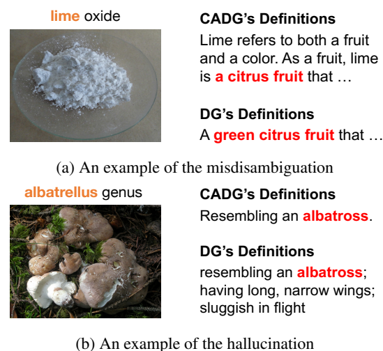
Figure 6: Examples of incorrectly generated definitions.
