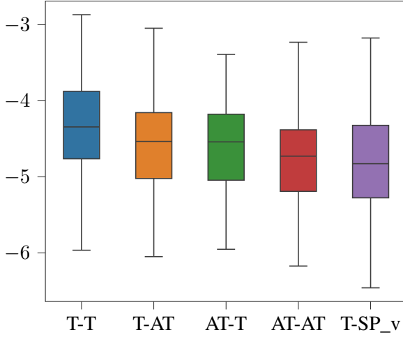
Figure 1: GPT-2 Sentence probability distribution
