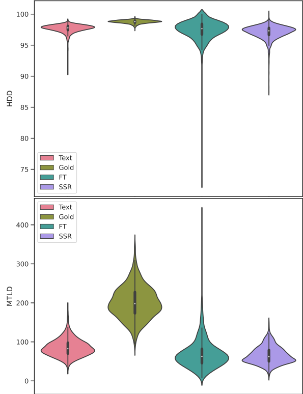
Figure 2: Distribution of lexical diversity. For HDD and MTLD \uparrow score is better.
