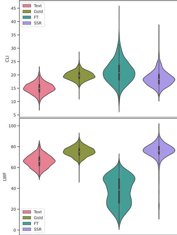
Figure 3: Distribution of readability scores. For CLI \downarrow score is better. For LWF \uparrow score is better.
