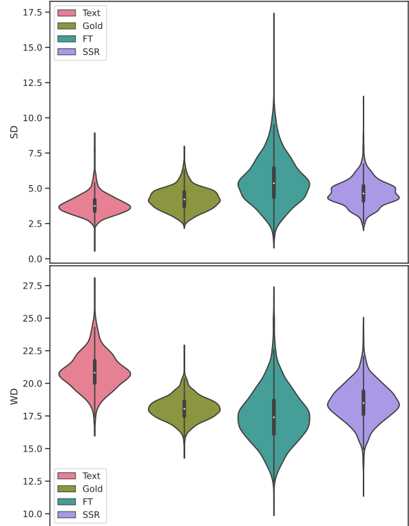
Figure 4: Distribution of density scores. For WD and SD \downarrow score is better.
