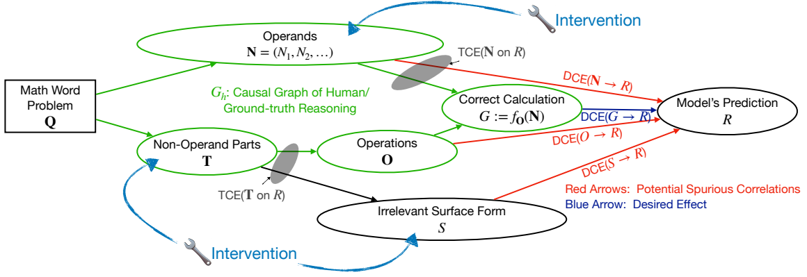
Figure 2: Causal graph of model predictions on math questions. We highlight the difference between a cognitively-inspired correct reasoning path ( G_h ) and the undesired effects that some factors might have on the model’s prediction (red arrows). By performing controlled interventions of the numerical values ( N ) and on the textual framing of the problem ( T , S ), we are able to quantify the causal effects of each factor.
