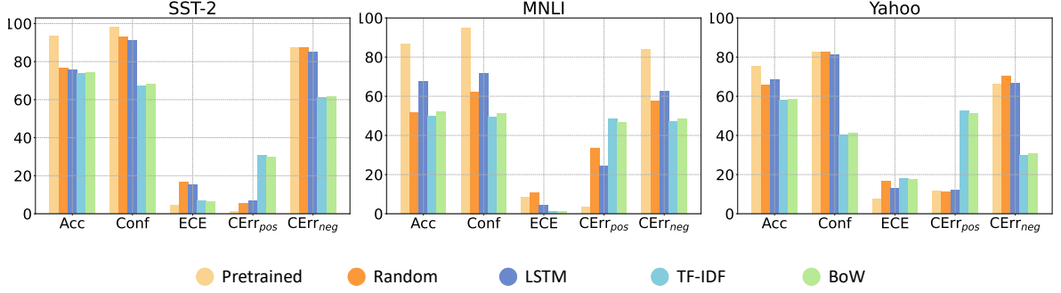
Figure 6: Results of the pretraining influence with T5.
