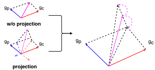
Figure 6: Intra-Layer Gradient Direction Projection. The w/o projection directly add the two gradient vectors, and the projection is to completely remove the conflicting parts of each other, and then add them. Our strategy is a fusion of them.
