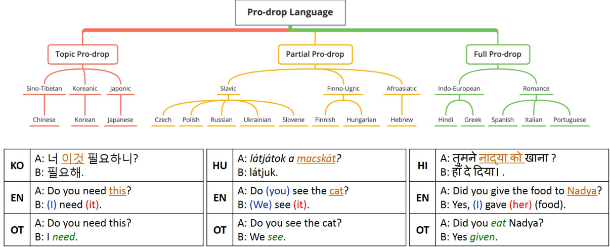
Figure 1: An overview of pro-drop languages by considering their typological patterns and language families. Example of ZP phenomenon in other languages (i.e. Korean, Hungarian and Hindi). Words in brackets are pronouns that are invisible in source language (implicit and explicit). The underlined words are corresponding antecedents. “EN” represents the human translation in English, which is a non-pro-drop language. “OT” is output translated by SOTA NMT systems with inappropriate translations .
