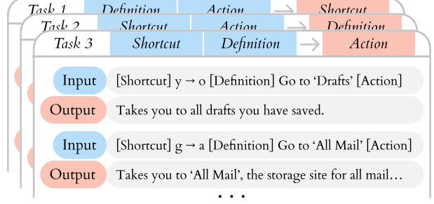
Figure 2: An algorithm to convert tables into tasks for FSL: Given the task of "Predict this column value given the other column values as input," each row in the table can be used as an example for that task.
