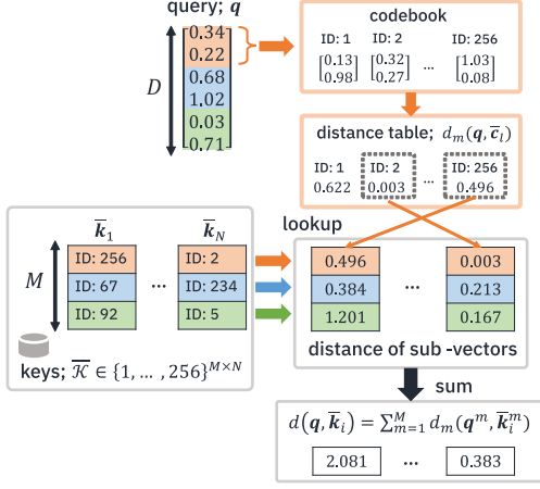
Figure 2: Distance computation using asymmetric distance computation (ADC).
