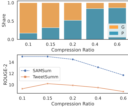
Figure 4: Comparison of compression ratios in DIONYSUS BASE using “Better ROUGE” strategy. The upper figure reflects the percentage of generated summaries (G) and “Principal” (P) at different compression ratios. The performance is measured using the ROUGE2-F1 metric on the SamSum and TweetSumm development sets.
