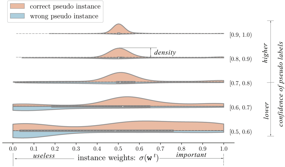
Figure 3: Distribution of activated weights ( \sigma(\mathbf{w}^t) ) over different kinds of pseudo instances.
