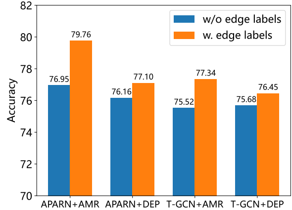
Figure 4: Accuracy of APARN and T-GCN on Twitter dataset with different parsed structures and edge labels.
