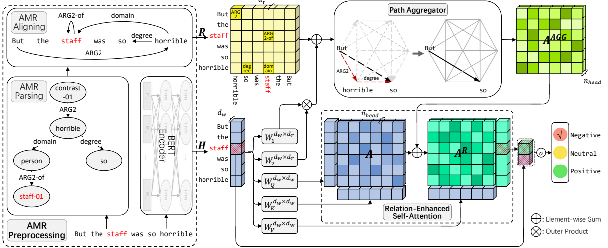
Figure 3: The overall architecture of APARN.
