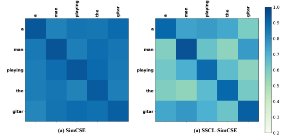
Figure 5: Token representation cosine similarity matrices from SimCSE and SSCL-SimCSE. Representations taken from the last layers of these models.
