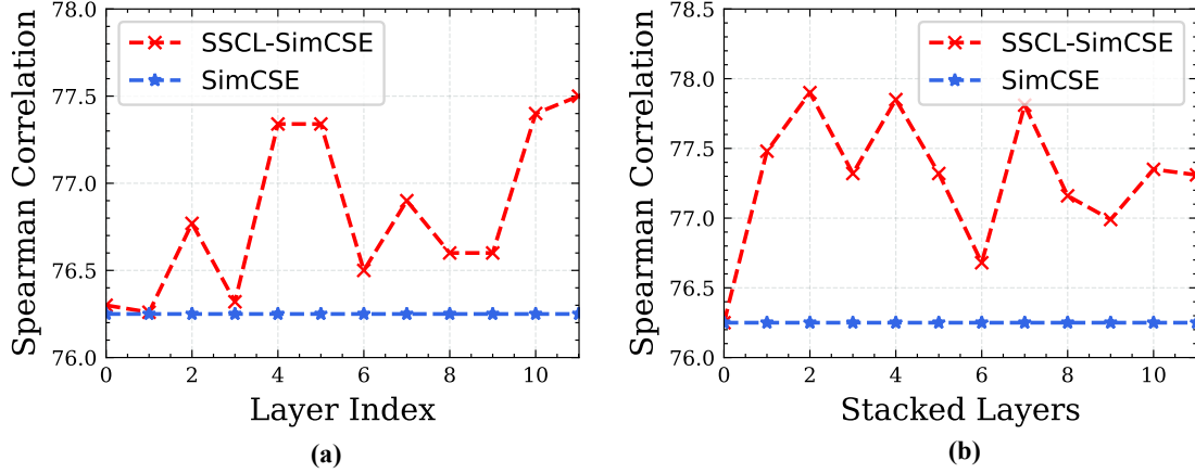
Figure 3: Layer negatives analysis of SSCL. (a) SSCL with different single layers to construct negatives, (b) SSCL with stacked different layers to construct negatives named Progressive SSCL. We report the average model performances in STS datasets.
