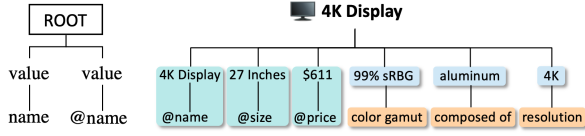
Figure 2: The abstract illustration of Attribute Tree (left) and an instantiated one describing the attributes of the example in Figure 1 (right). The attribute names starting with “@” represent those stemming from the schema.
