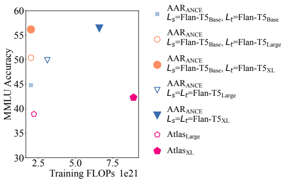
Figure 3: Training FLOPs of AAR ANCE and Atlas.
