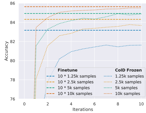
(b) Effect of Dataset Size per Contributor
