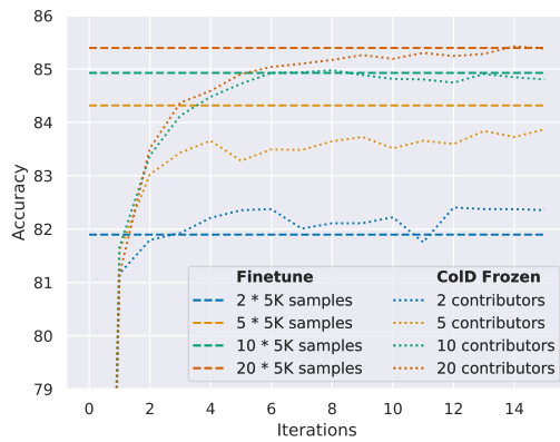
(c) Effect of #Contributors
