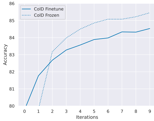
(a) Effect of Additional Data
