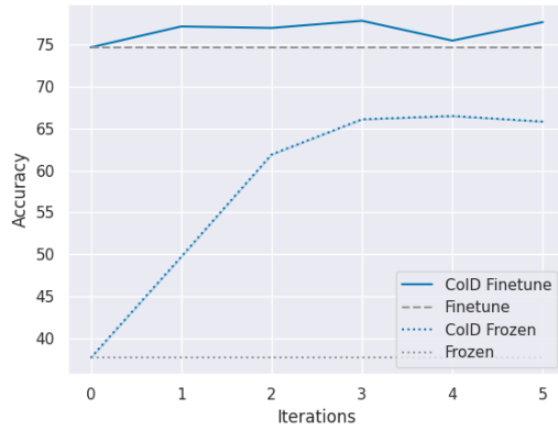
Figure 8: CoLD Fusion on T5. We replicate the main experiment (§5) on a smaller scale. Like in RoBERTa, both CoLD and CoLD-Frozen lines keep increasing with the iterations.
