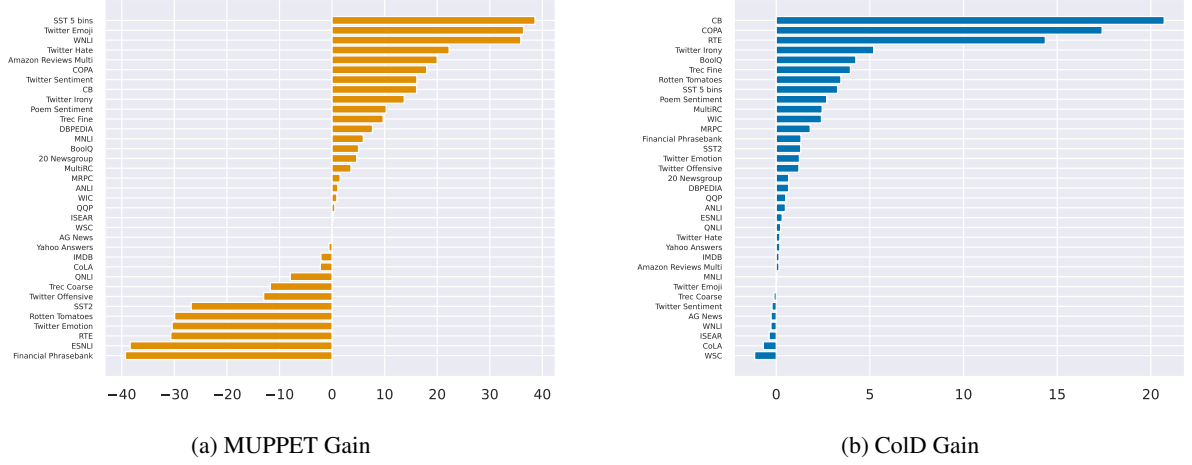
Figure 7: Gains of MUPPET/CoLD over finetuning on the pretrained model. CoLD is much more consistent, with less datasets that lose from changing from pretrained to CoLD and smaller negative effects on them. MUPPET however has larger maximal gain when it does show gains.
