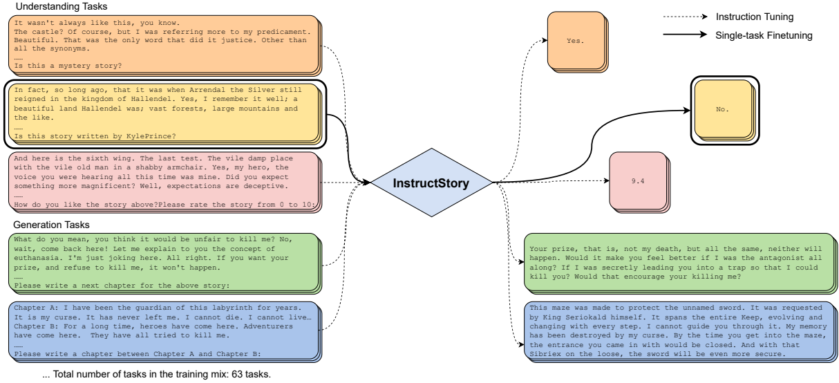
Figure 2: INSTRUCTSTORY undergoes a two-stage training process. In stage 1 ( --\rightarrow ), we instruction tune the model on 63 story tasks to improve generalization to unseen zero-shot and few-shot tasks. In stage 2 ( \rightarrow ), we perform single-task finetuning on each fully-supervised task to optimize performance on specific tasks.
