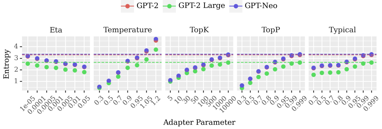
Figure 6: Average entropy of the distribution \tilde{p}_\theta(\cdot | \mathbf{y}_{<t}) for different sampling adapter-hyperparameter combinations. Dashed lines correspond to the entropy of the unmodified distribution.
