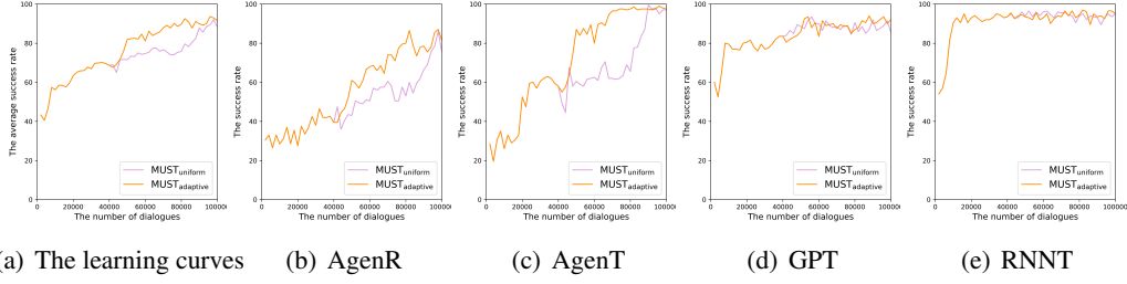
Figure 2: The learning curves of Sys-MUST uniform and Sys-MUST adaptive . (a) shows their average success rates tested with all user simulators (AgenT, AgenR, RNNT, and GPT). The success rates of them tested with each user simulator are shown in (b)-(e).
