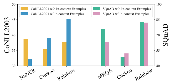
Figure 5: In-context tagging ability emerges in Cuckoo but not in IE models pre-trained by other resources.
