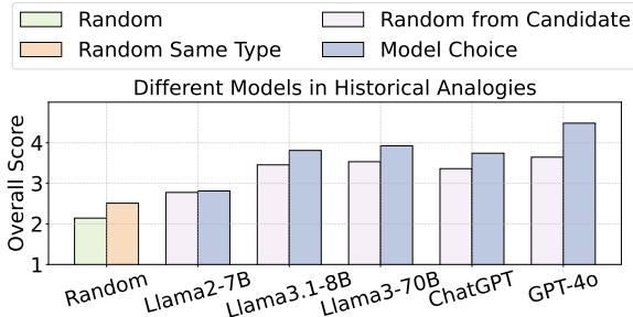
Figure 7: Performance of different models in historical analogies, including proposing candidate sets and selecting analogous event.
