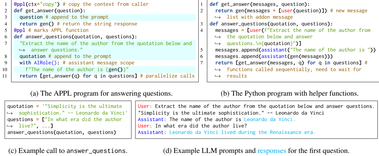
Figure 2: (a) The APPL program for answering multiple questions about a quotation by first extracting the author’s name. In this APPL program, the @ppl marks the function to be APPL function, which provides a context that interactive expression statements (highlighted lines) can be interacted with. Passing the context across APPL functions is implicitly handled along with function calls, mimicking the process of stack frame management. The gen function requests an LLM generation using the prompts stored in the context, with other optional arguments following the OpenAI’s API (OpenAI). For instance, the gen in line 4 uses the prompt composed by (highlighted) lines 7,8,10 (since context is copied), and 3. The LLM generation is computed asynchronously and only synchronizes when the value is needed, therefore independent calls are automatically parallelized as shown in line 11. (b) A Python program implementing the same function uses more codes, even with the helper functions. Furthermore, extra codes are needed to parallelize get_answer function calls. (c) Example usage for the program and (d) its corresponding LLM prompts and example responses.
