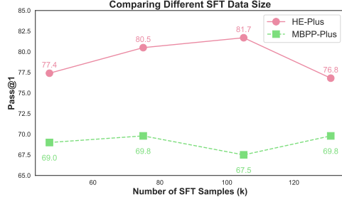
Figure 3: Comparison of performance across different numbers of instruction fine-tuning samples synthesized by our ToE framework.
