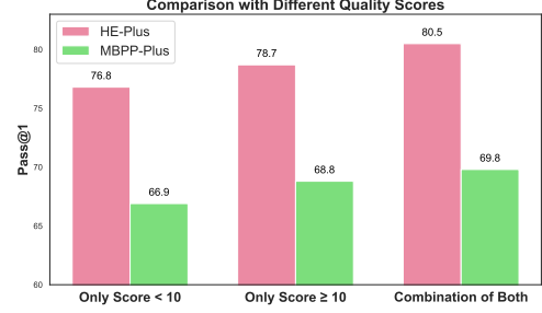
Figure 5: Comparison of performance across different quality scores.
