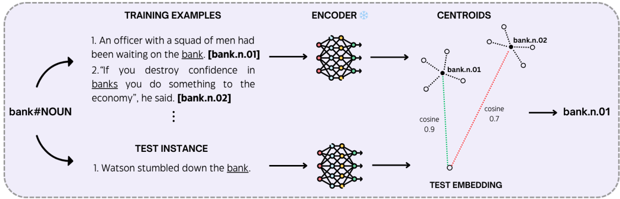
Figure 1: A graphical representation of the proposed methodology. Given a target lemma, we use its training examples to compute sense-level centroids by means of a frozen transformer encoder \mathcal{M} . Then, for disambiguating a test instance, we select the sense associated with the centroid that maximizes the cosine similarity score. Note that, for the sake of visualization, we focus only on the first two senses of bank#NOUN in this example.
